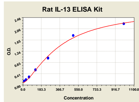
Figure 1: IL-13 Standard Curve. Using the Rat IL-13 ELISA Kit, O.D. data was graphed against IL-13 protein concentration. The TMB reaction was incubated at 37°C for 17 min.
